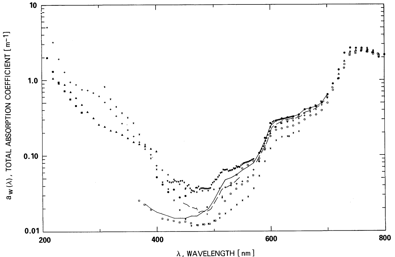
Fig. 1. Total absorption coefficient for pure freshwater [ a_w(\lambda)(\text{m}^{-1}) ] vs wavelength [ \lambda(\text{nm}) ] as given by various authors: solid line, Morel and Prieur 8 ; dashed line, Tam and Patel 10 ; \nabla , Querry et al. 7 ; 1, 2, Hass and Davison 9 ; \times , Sawyer 26 ; + , Dawson and Hulburt 27 (200–400 nm) and Hulburt 28 (400–700 nm); \blacktriangle , Lenoble and Saint-Guilly 31 ; \square , James and Birge 29 ; \circ , Clark and James 30 ; \triangle , Curcio and Petty 40 ; \bullet , Sullivan 32 ; \blacksquare , Armstrong and Boalch. 22
