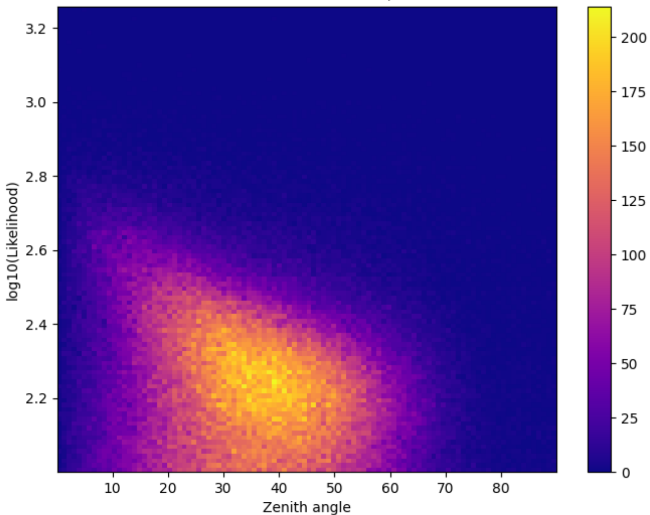
likelihood zeniths correlation, Lik>100
