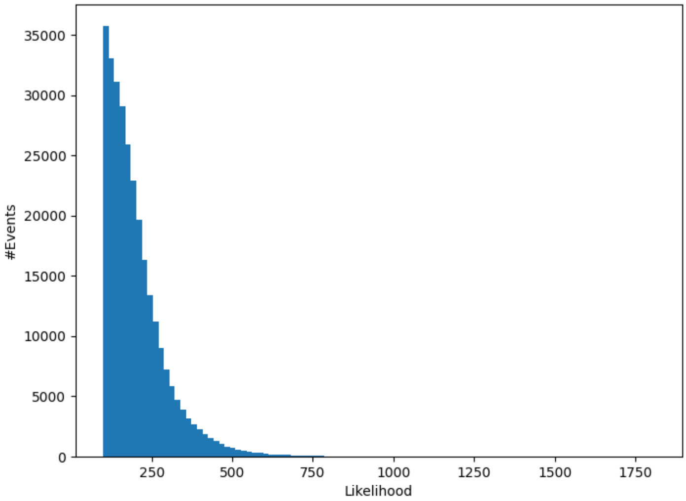
Event likelihood distribution, Lik>100
