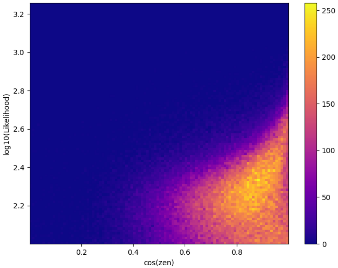
likelihood cos(zen) correlation, Lik>100
