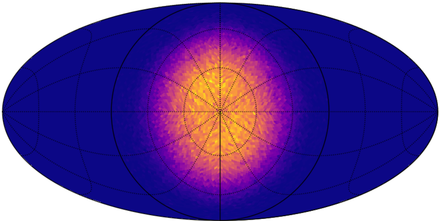
Map, Likelihood > 100, zenith < 90
