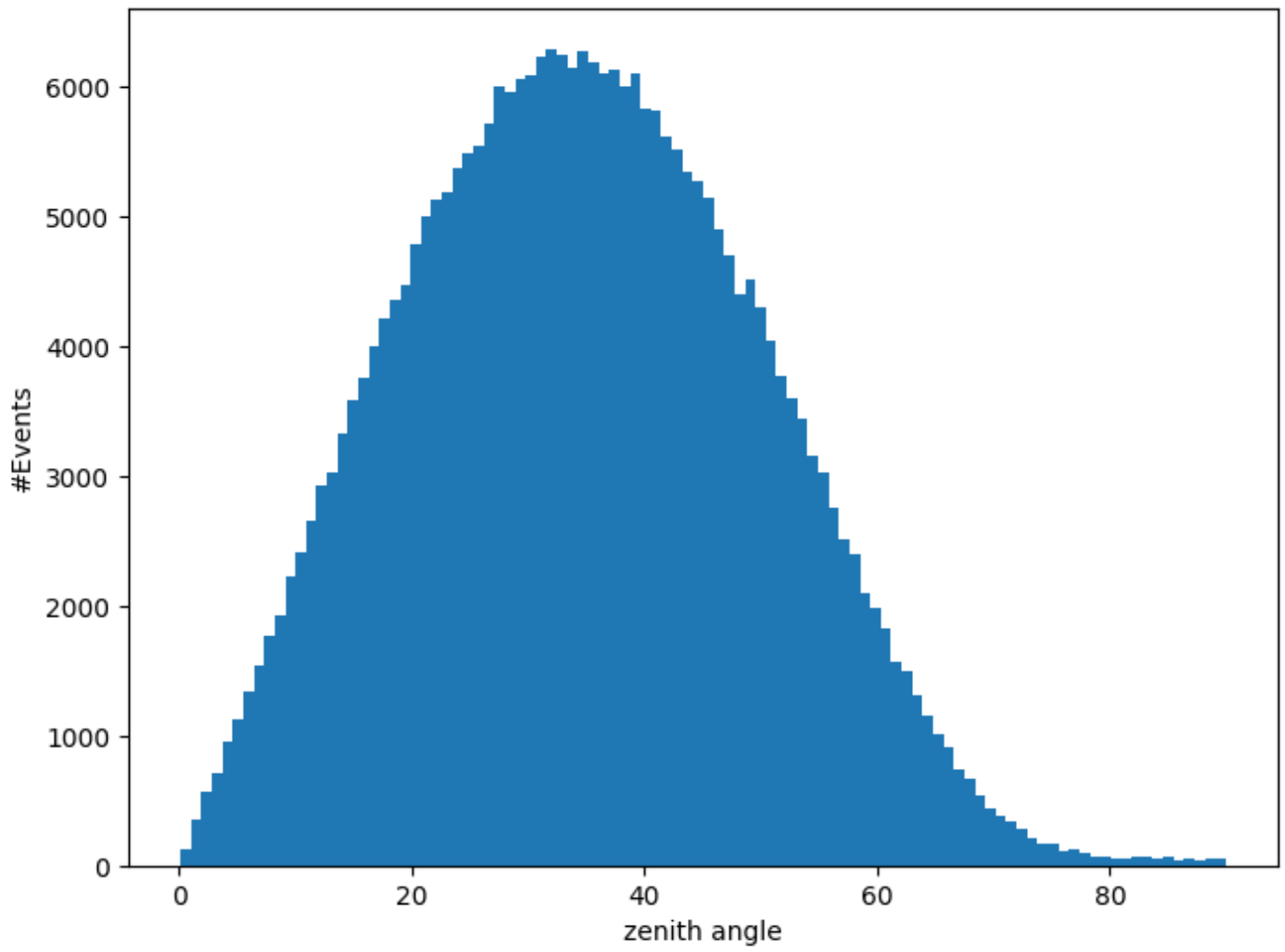
Event zenith distribution, Lik>100
