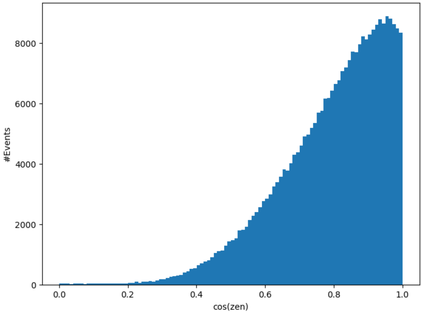
Event distribution, Lik>100
