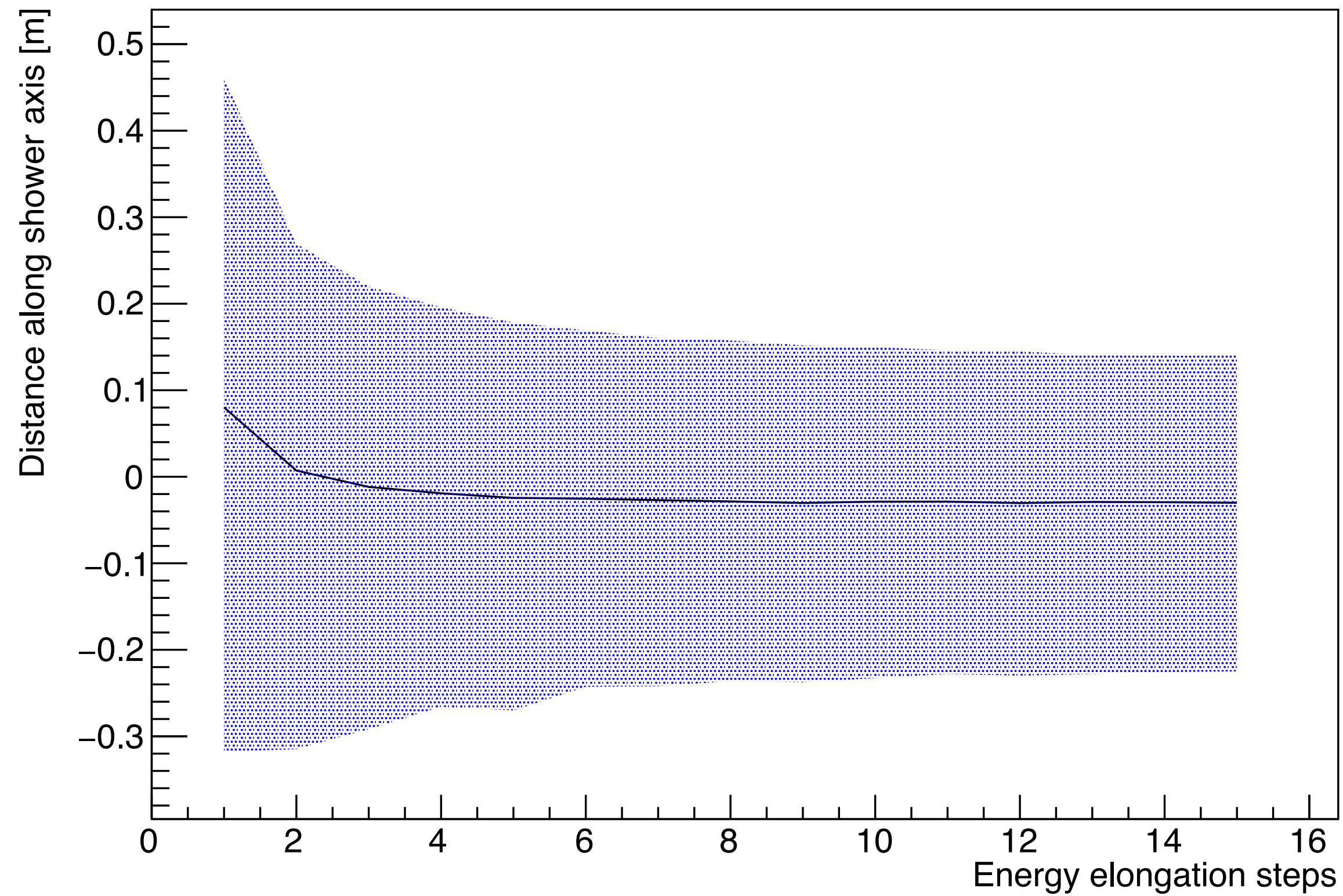
Vertex fit resolution
