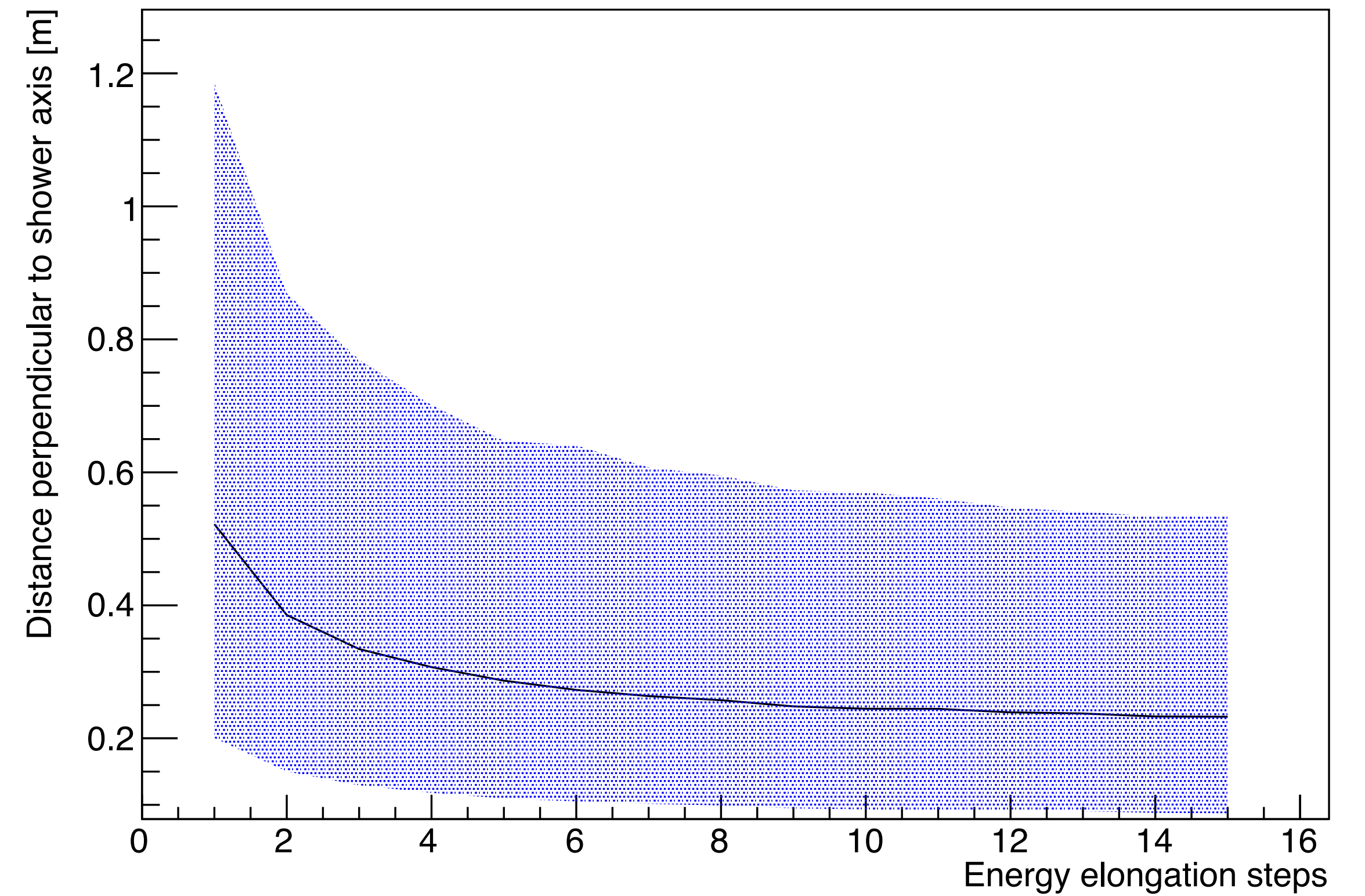
Vertex fit resolution
