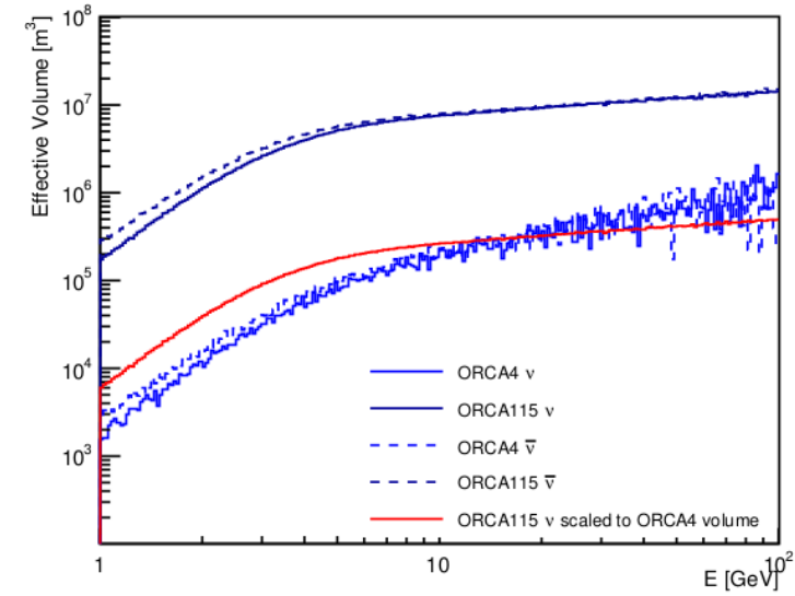
Effective volume: e-cc
