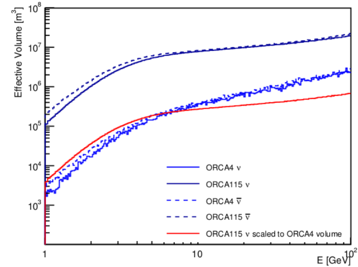
Effective volume: \mu -cc
