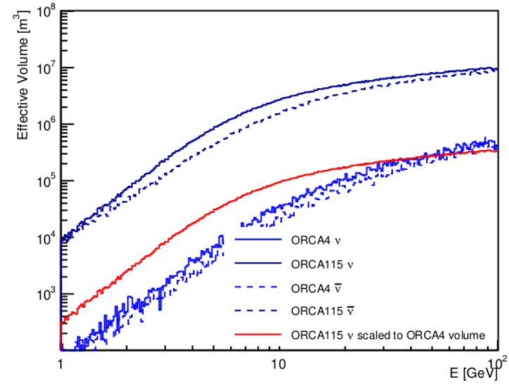
Effective volume: \mu -nc
