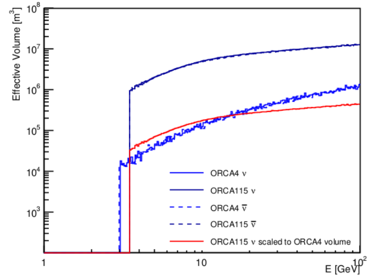
Effective volume: \tau -cc
