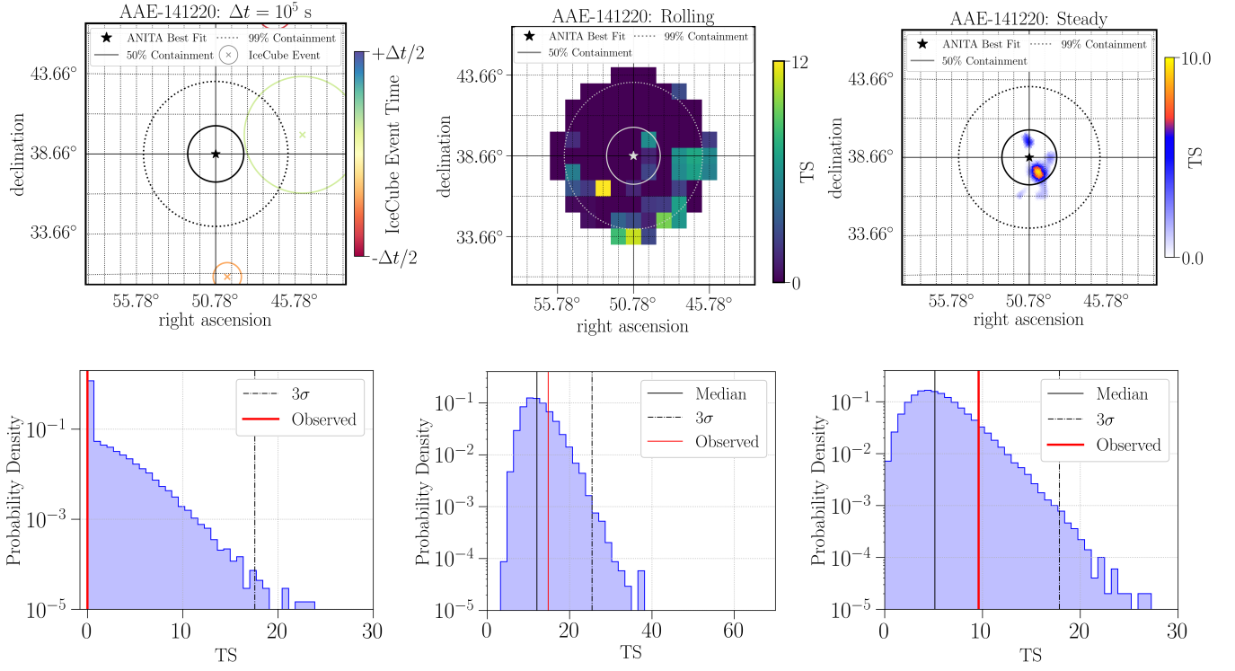
Figure 1. Skymaps (top) and TS distributions (bottom) for AAE-141220 for the prompt (left), rolling (middle), and steady (right) analyses. Observed TS values (shown in red) are compared to distributions from time-scrambled data realizations to quantify the significance. In the prompt analysis skymap, the best-fit location of each IceCube event is represented with an \times , and the size of the circle represents the uncertainty (90% containment) on the event’s reconstruction, with color representing the IceCube event arrival time relative to the ANITA event. In the rolling and steady analysis skymaps, color reflects the TS values defined in sections 3.2 and 3.3 respectively.
