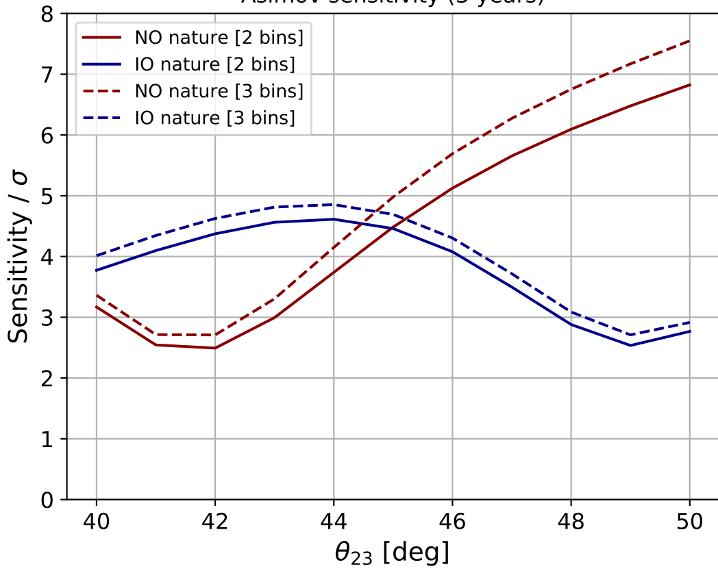
Asimov sensitivity (3 years)
