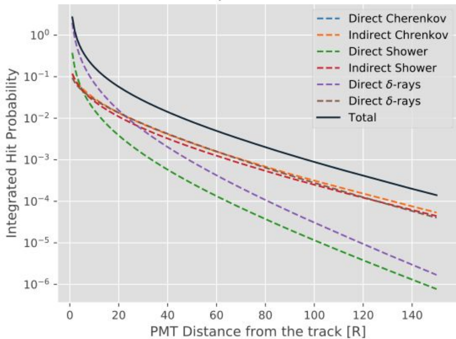
IHP at \phi = 0.00 \theta = 0.00
