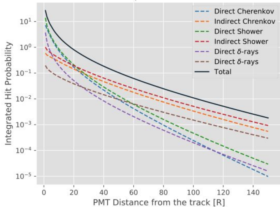
IHP at \phi = 3.10 \theta = 2.20
