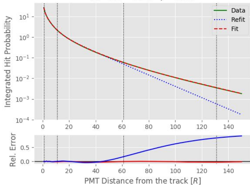
IHP at \theta = 3.10 \phi = 2.20
