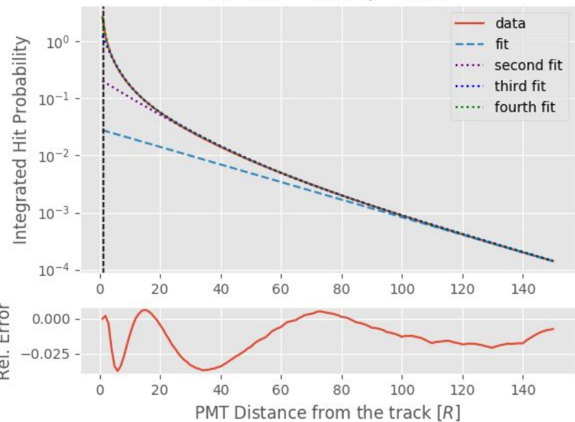
IHP at \theta = 0.00 \phi = 0.00
