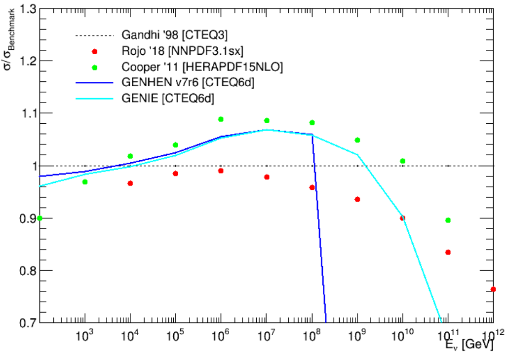
\nu_\mu CC cross section
