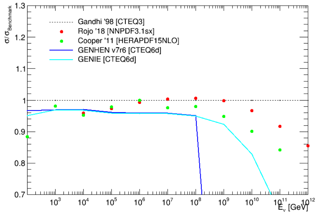
\nu_\mu NC cross section
