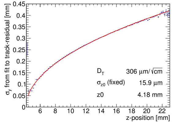
Figure 8: Measured hit resolution in pixel plane (blue points) fitted with the resolution according to equation (2) (red line).
