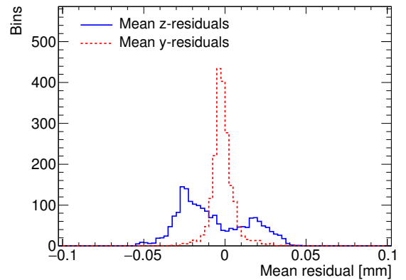
Figure 12: Distribution of the mean residuals from 4 \times 4 bins within the selected region.
