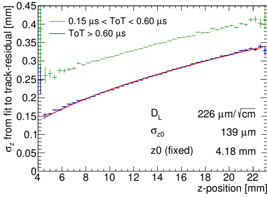
Figure 9: Measured hit resolution in drift direction split by ToT. The hits with a ToT above 0.60 \mu\text{s} (blue points) are fitted with the resolution according to equation (2) (red line).
