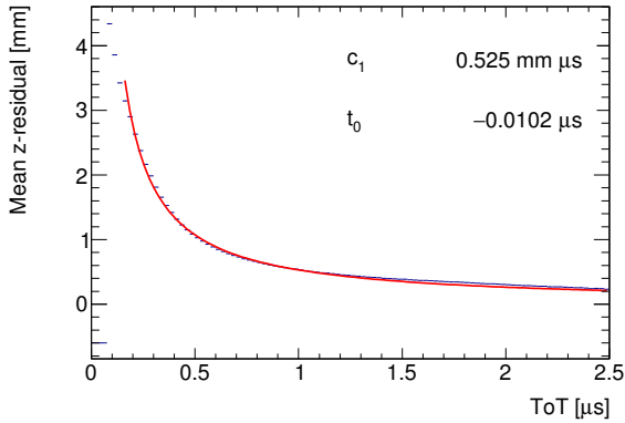
Figure 6: Mean z -residual without time walk correction as function of ToT, fitted with equation 1.
