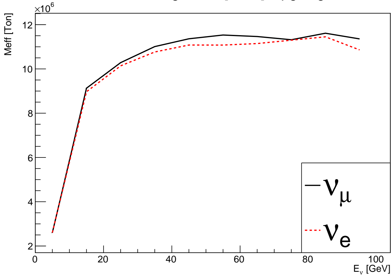
cos \theta average Meff [Tons], upgoing
